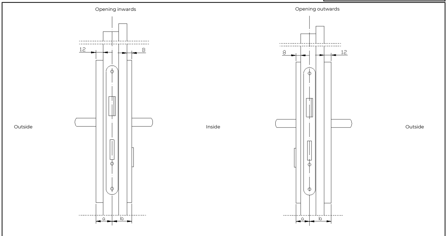
Above drawing applies to "Porta Agat", "Porta Opal", "Porta Granit", "Royal" and "Porta Safe".
