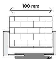
STANDARD RANGE adjustment without shortened architrave tongue
