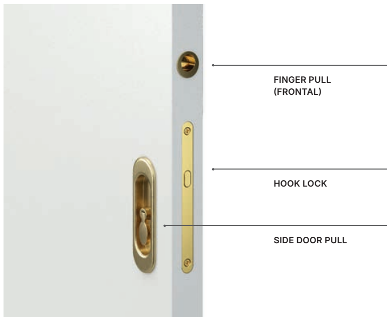
HOOK LOCK WITH KEY OR BATHROOM LOCK WITH SIDE AND FRONT DOOR PULLS, FOR SLIDING DOORS Gold, matte gold, silver, matte silver, black
