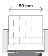
MINIMUM RANGE adjustment after shortening the architrave tongue
